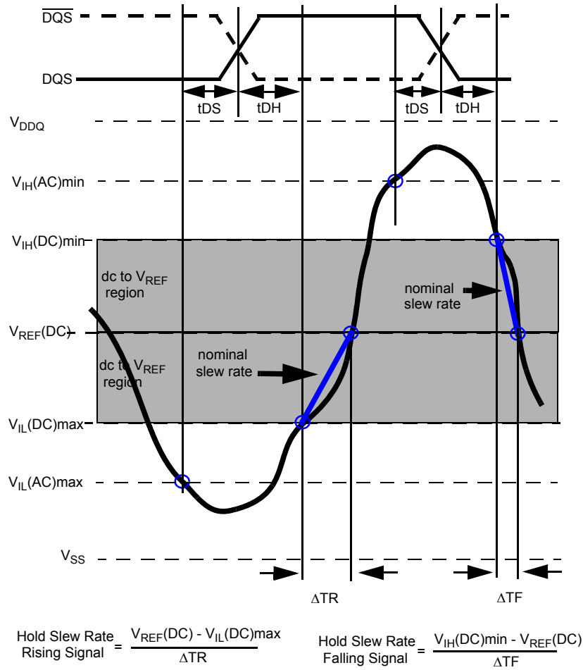
Figure 9 - Illustration of nominal slew rate for t DH (differential DQS, \overline{\text{DQS}} )
