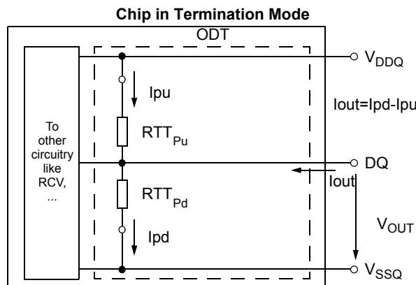
Figure 12. On-Die Termination : Definition of Voltages and Currents
