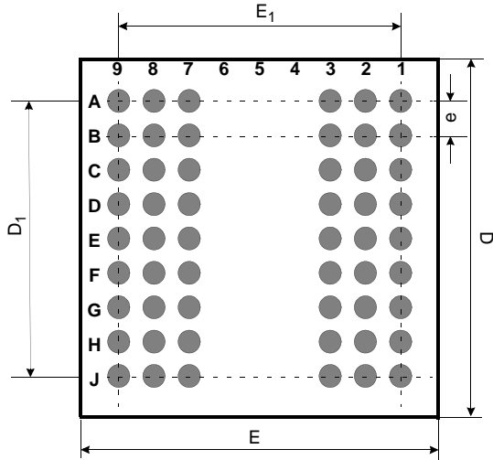
< Bottom View *1 >
