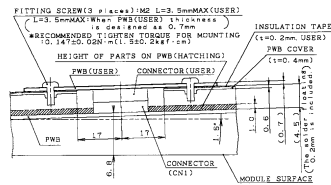
Fig 1. OUTLINE DIMENSIONS (LQ104S1DG61)
