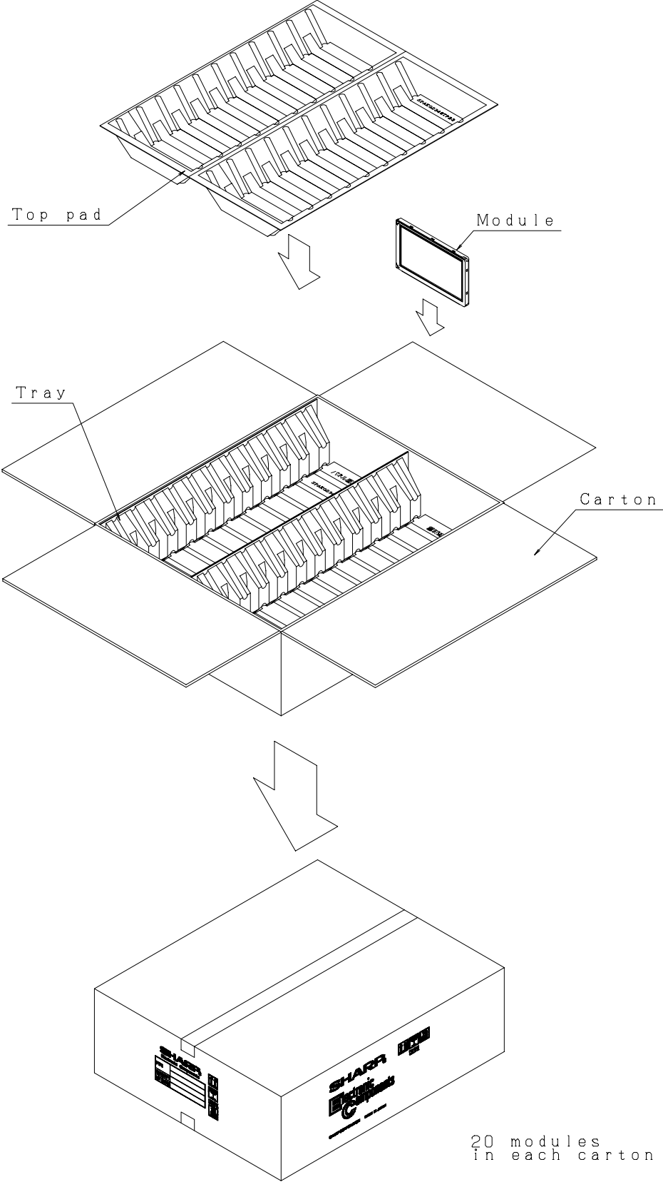
Fig4-1 Packing form
