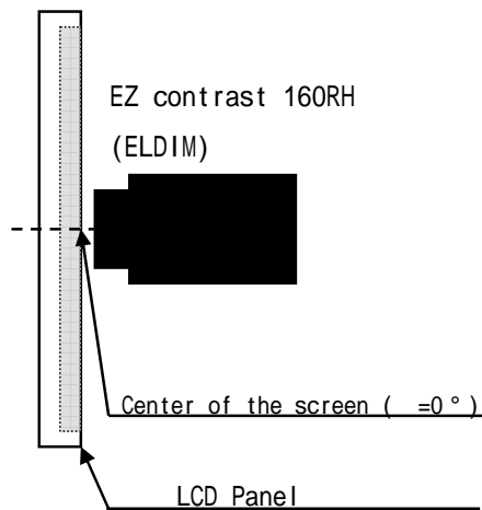
[Note 1] Measuring Viewing Angle Range
