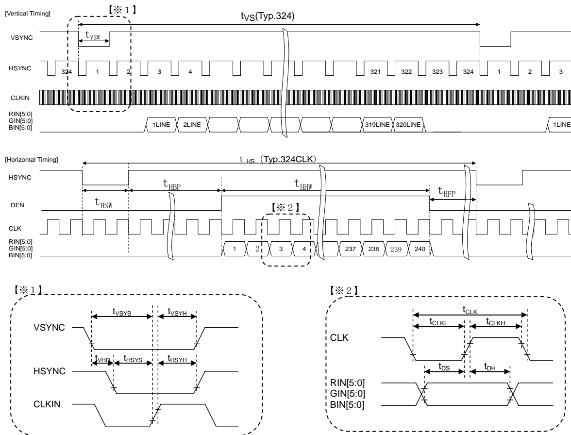
Fig 7-4 LCDIF signal timing in Portrait QVGA mode
