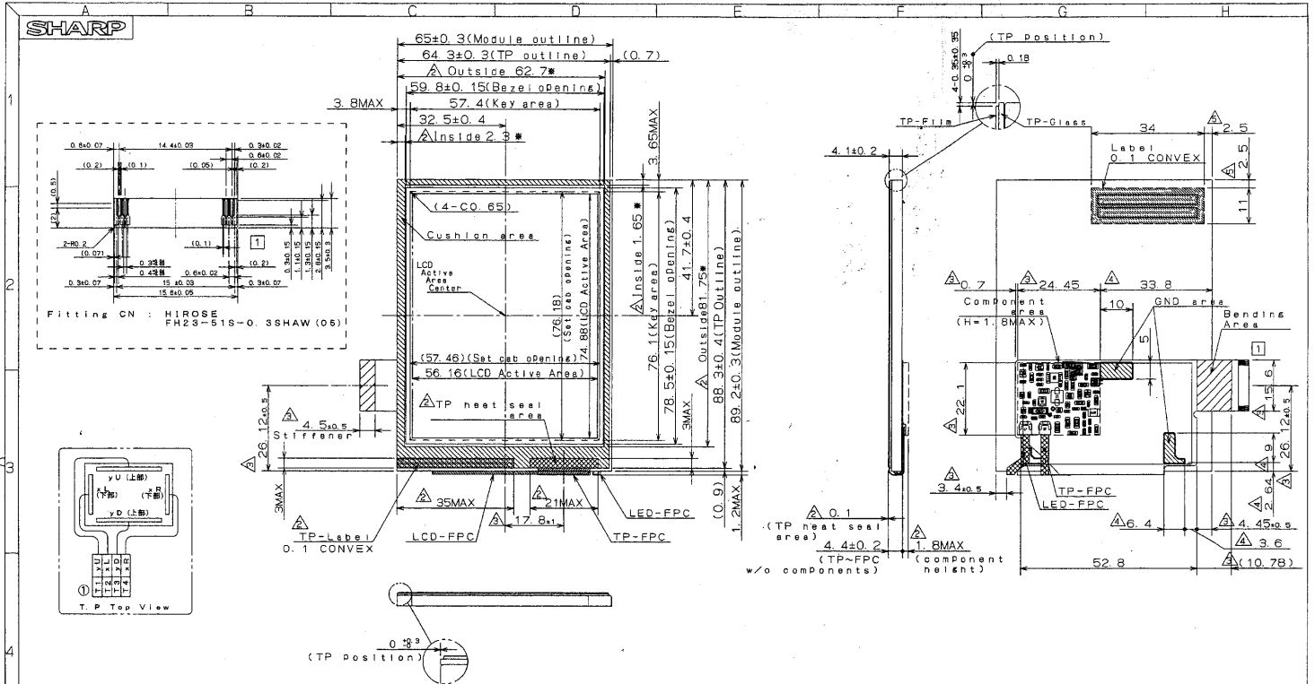
Fig. 1 Outline dimensions
