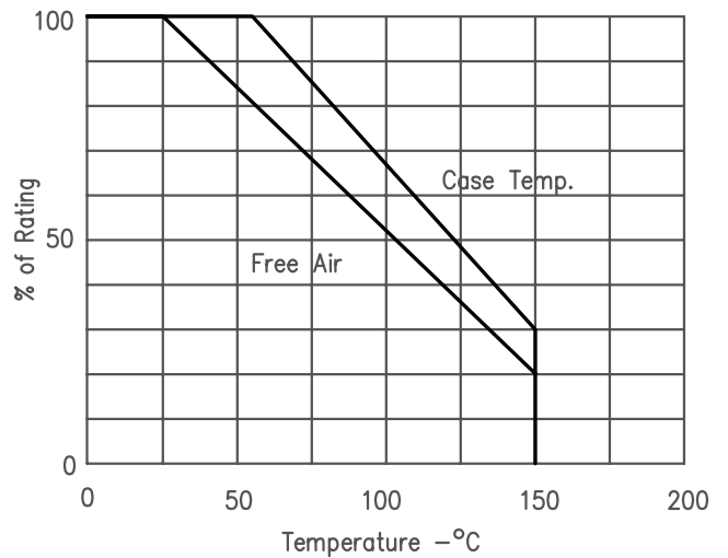
Figure 4 Current Derating
