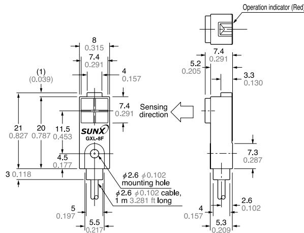
GXL-8F type Sensor
