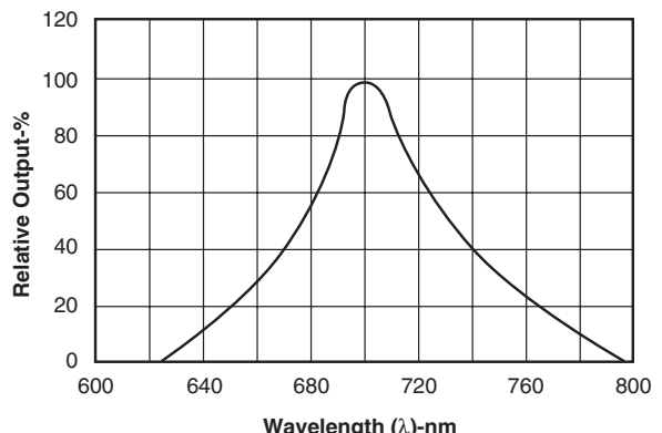
Fig. 2 Spectral Response
