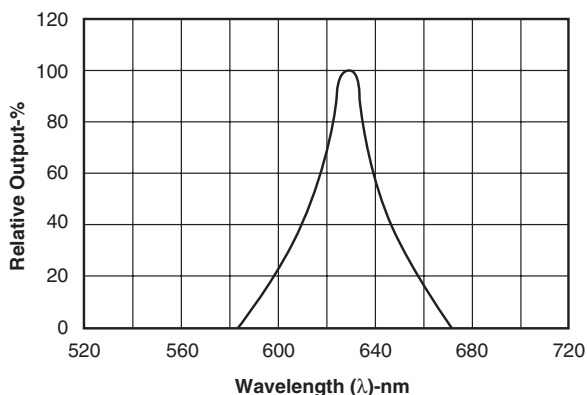
Fig. 2 Spectral Response
