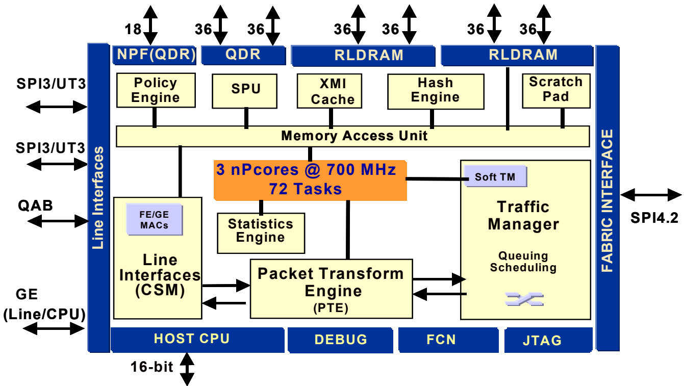
nP3700 Block Diagram
