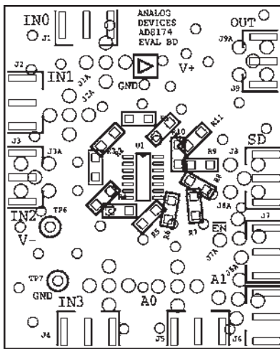
Figure 6. EVAL-AD8174EB Component Side Silkscreen
