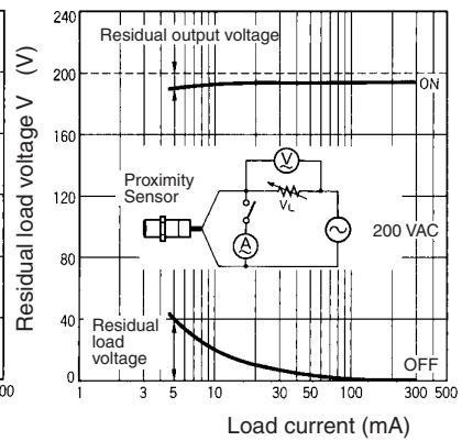
200 VAC
