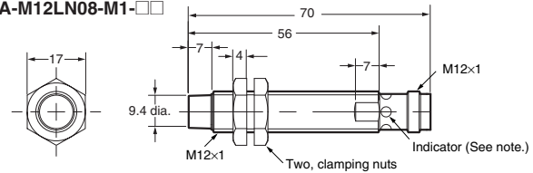
E2A-M12LN08-M1-□□
