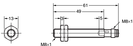
E2A-S08LS02-M5-□□
