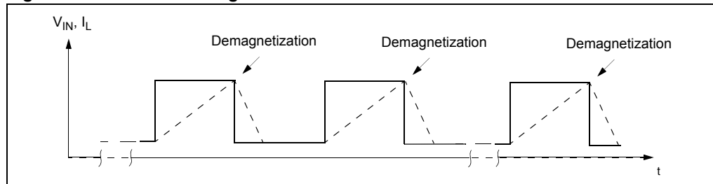
Figure 35. SOT-223 demagnetization
