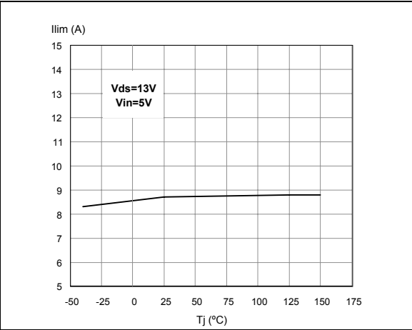
Figure 28. Normalized current limit vs junction temperature
