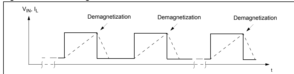
Figure 33. DPAK demagnetization
