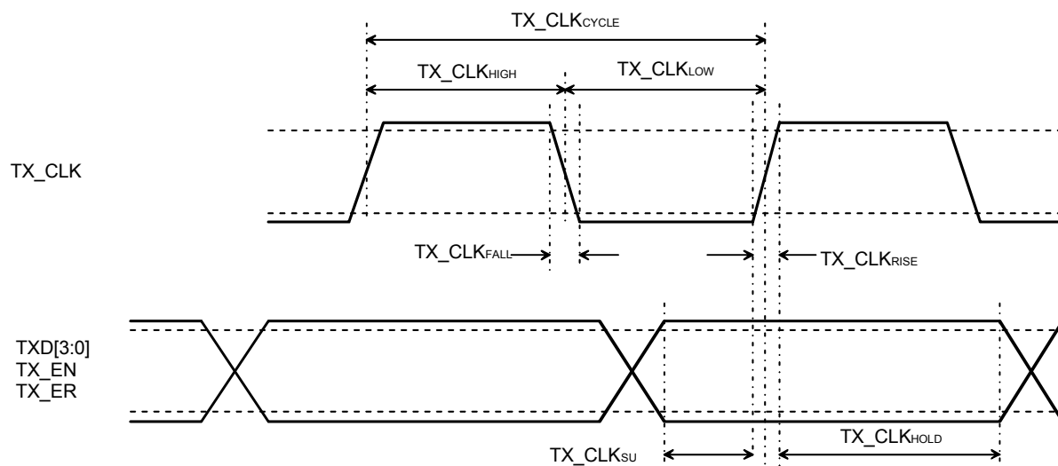
Figure 23. MII 10Base-T Transmit Timing
