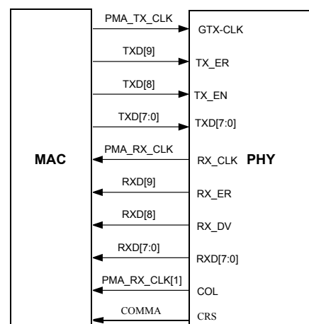
Figure 13. Ten-Bit Interface
