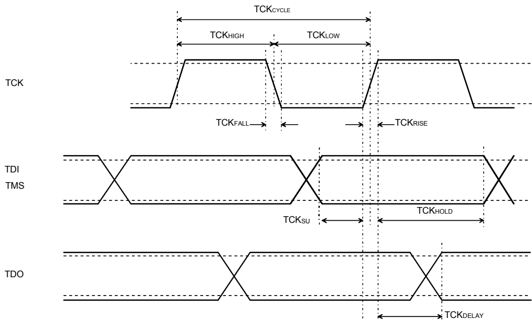
Figure 28. JTAG Timing
