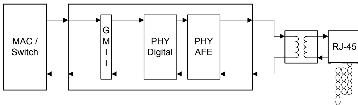
Figure 5. External Cable Loopback
