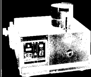
Stripper Crimper, Type AM 05 Part Number 1105866-1 Electro-Pneumatic Machine for Terminating Loose-Piece Screw Machined Male and Female Contacts
