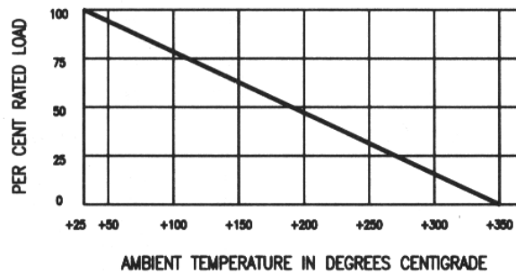
Figure 1 Series VPR Derating
