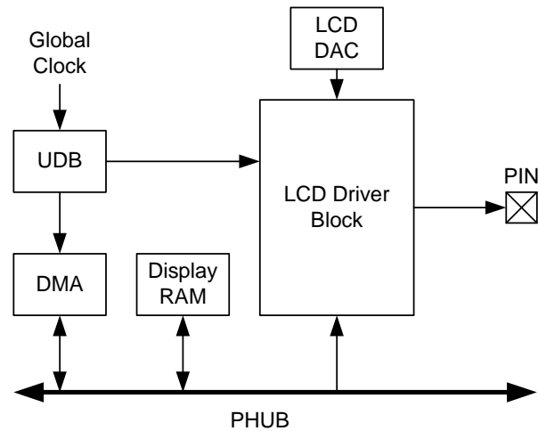
Figure 8-5. LCD System
