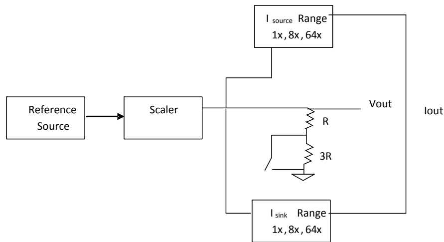
Figure 8-6. DAC Block Diagram
