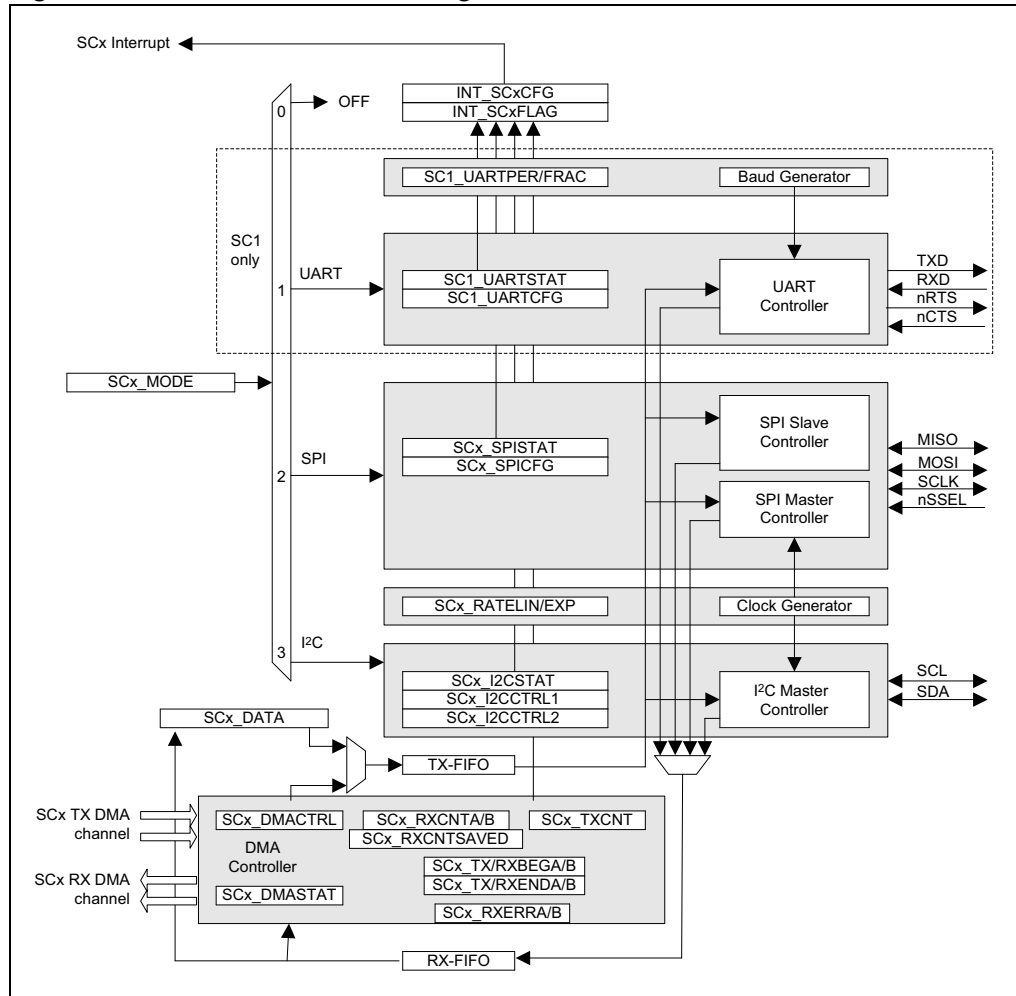
Figure 9. Serial controller block diagram
