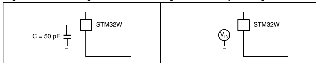
Figure 53. Pin loading conditions
