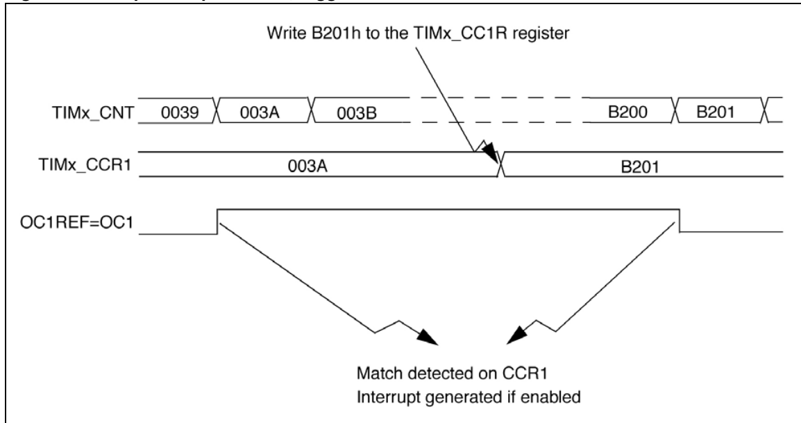
Figure 34. Output compare mode, toggle on OC1
