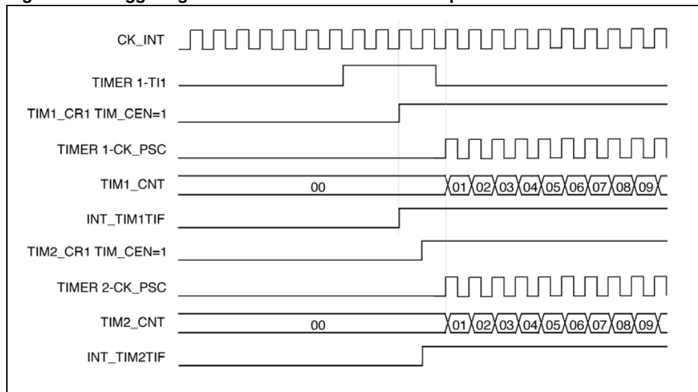
Figure 49. Triggering timer 1 and 2 with timer 1 TI1 input
