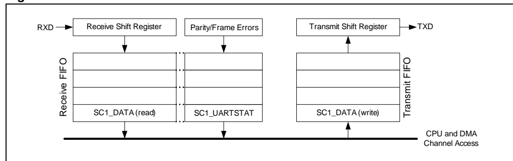
Figure 12. UART FIFOs
