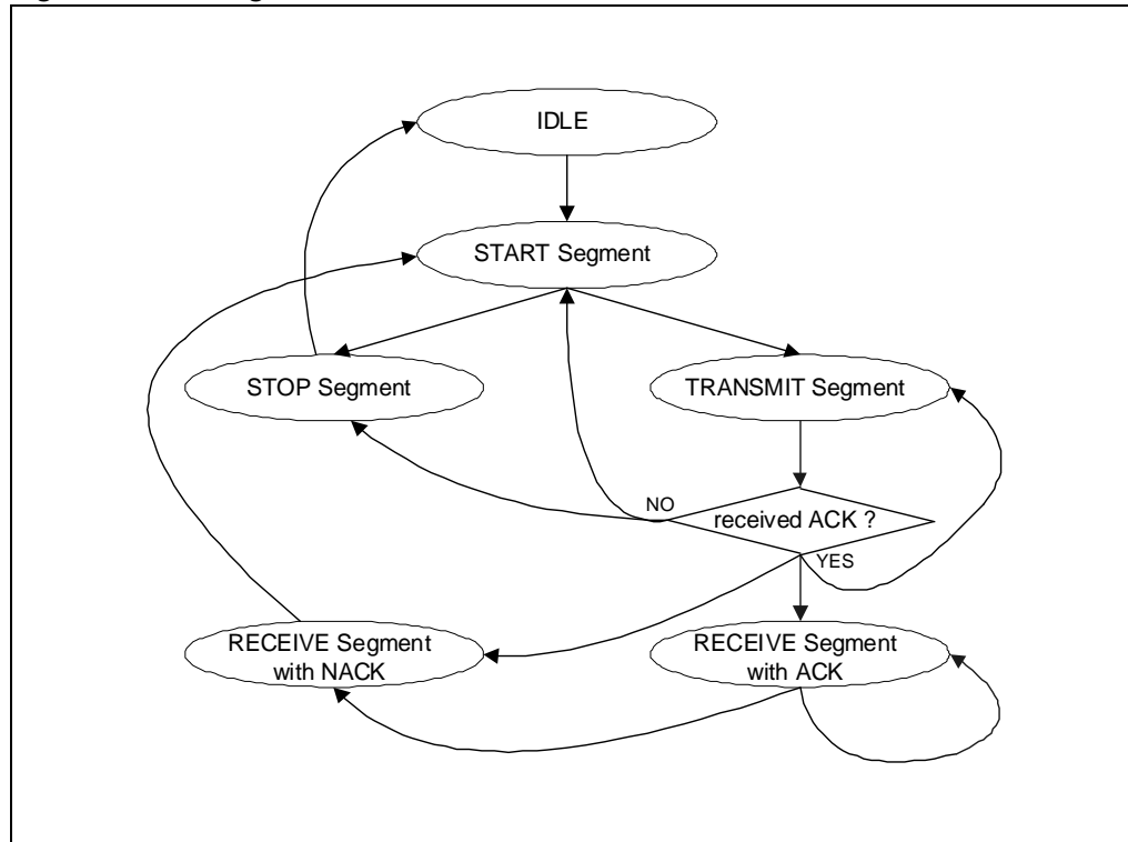
Figure 10. I 2 C segment transitions
