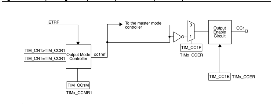
Figure 32. Output stage of capture/compare channel (channel 1)
