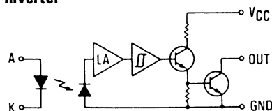
OPB903/OPB913 (Open-Collector Output) Inverter
