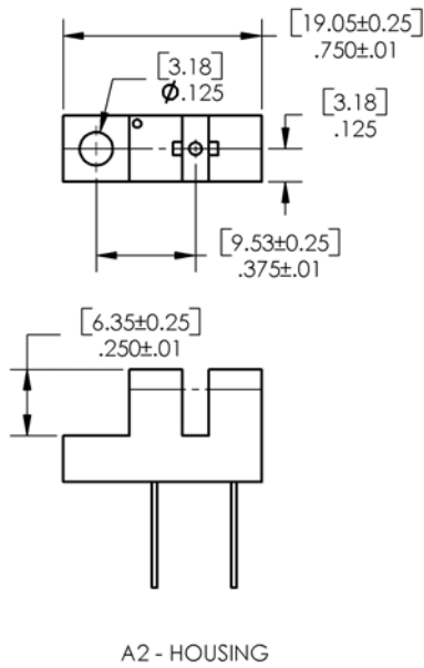
A2 - HOUSING
