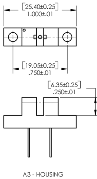
A3 - HOUSING
