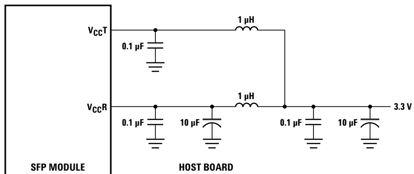
Figure 3. Recommended Application Configuration
