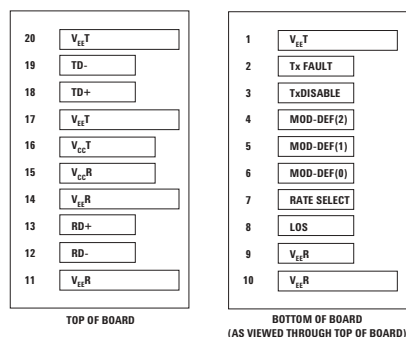
Figure 2. Connection Diagram of Module Printed Circuit Board
