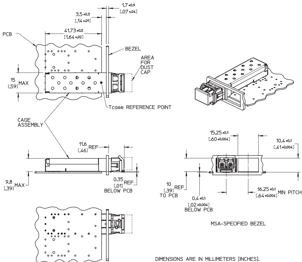
Figure 7. Assembly Drawing
