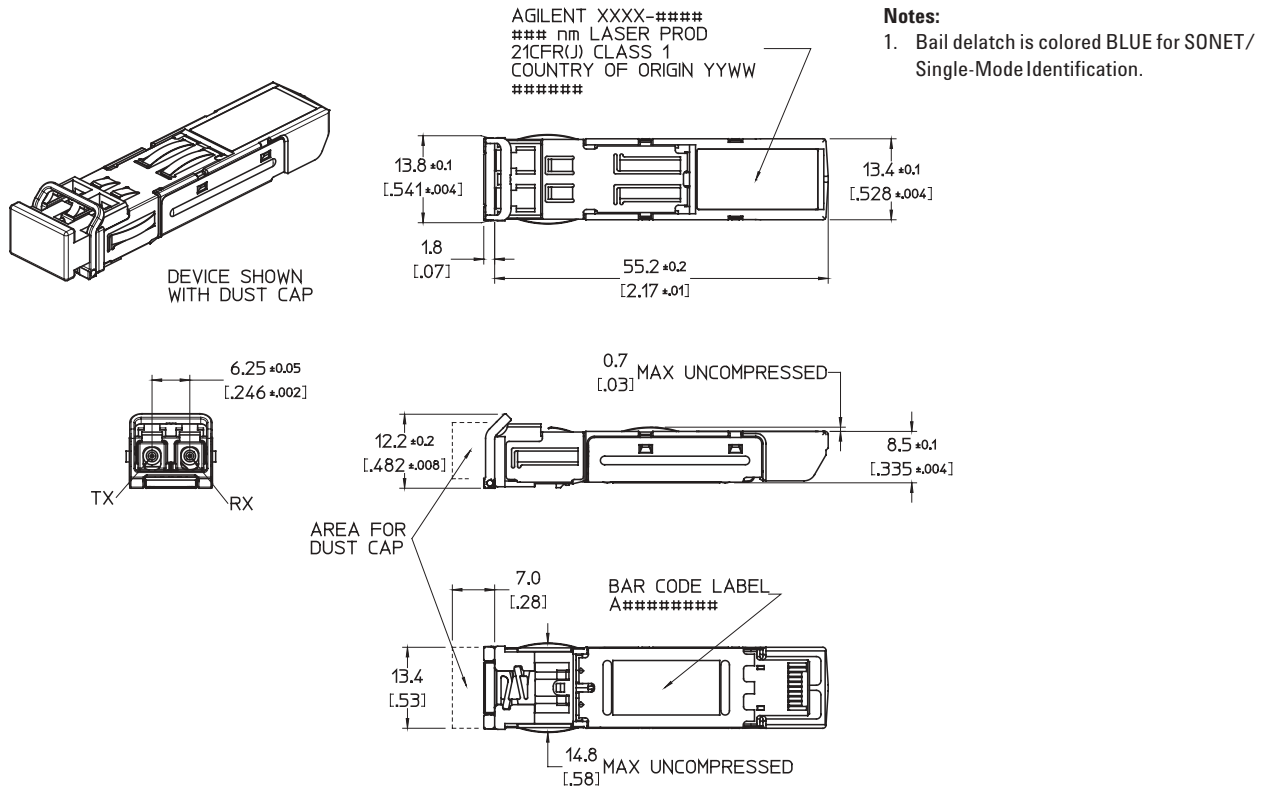
Figure 6. Module Drawing
