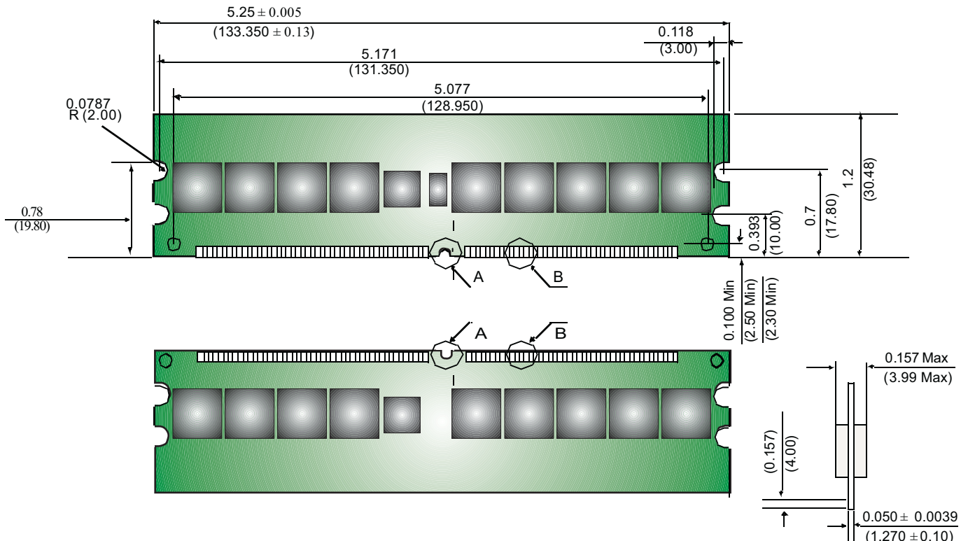
Figure 1: KVR333S4R25/1G 184-Pin DIMM
