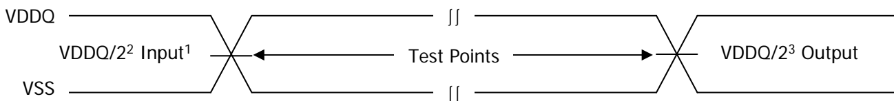
Figure 8. AC Input/Output Reference Waveform
