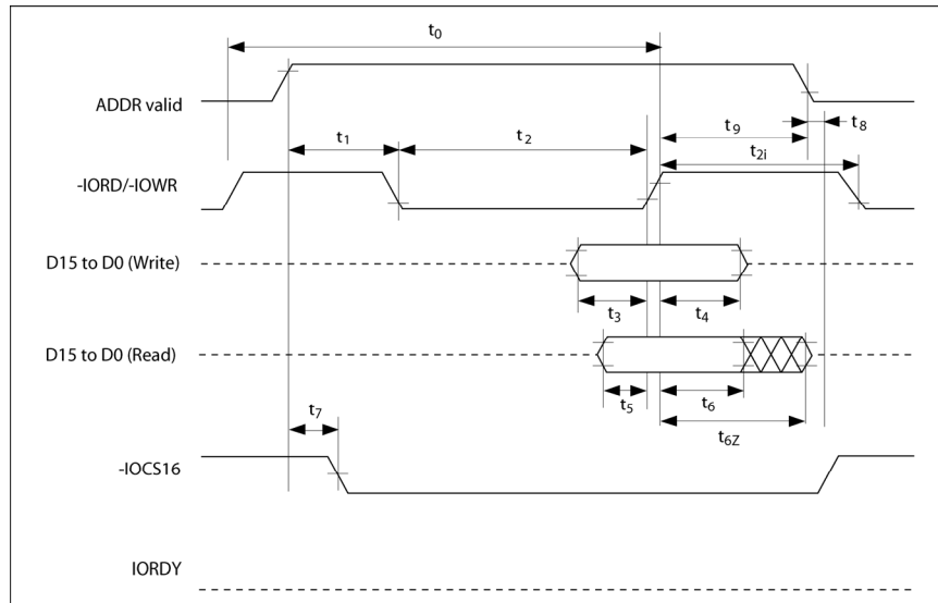
Figure 4: True IDE Mode Register and PIO Access Timing Diagram
