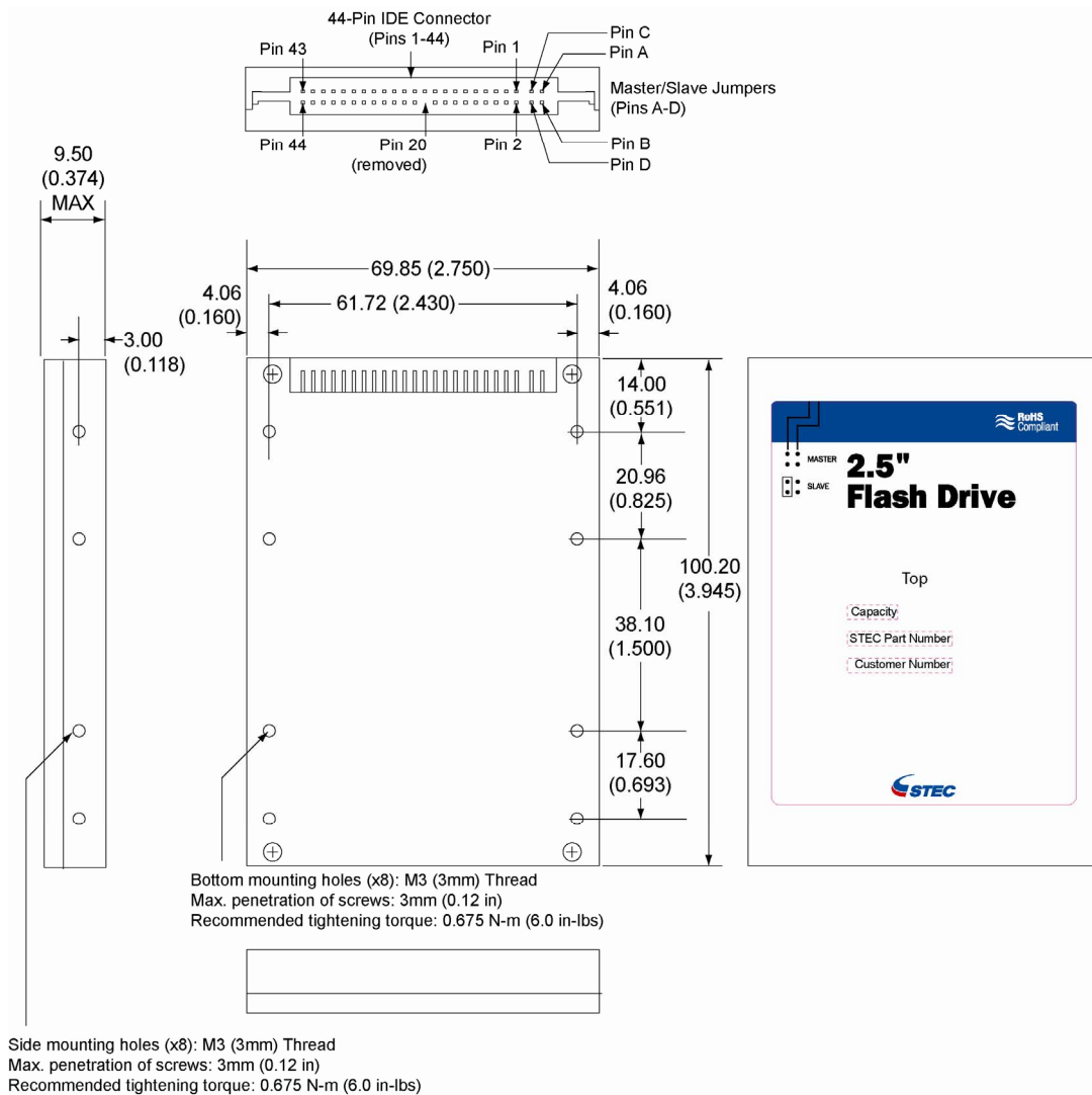
Figure 2: Mechanical dimensions of the 2.5-inch drive
