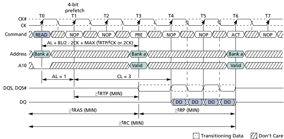
Figure 49: READ-to-PRECHARGE – BL = 4
