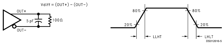
FIGURE 3. DS90CF583 (Transmitter) LVDS Output Load and Transition Times
