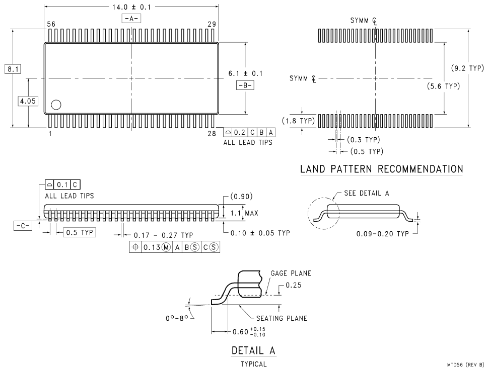
56-Lead Molded Thin Shrink Small Outline Package, JEDEC Order Number DS90CF583MTD or DS90CF584MTD NS Package Number MTD56
