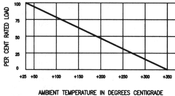
Figure 1 Series VP & VK Derating
