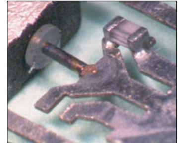
Anode, fuse and leadframe assembly
