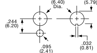
MTA8106DVRA Vertical Actuation
