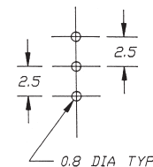
P.C. MOUNTING
