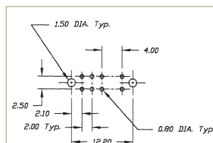
P.C. MOUNTING
