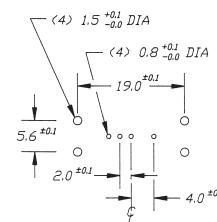
P.C. MOUNTING
