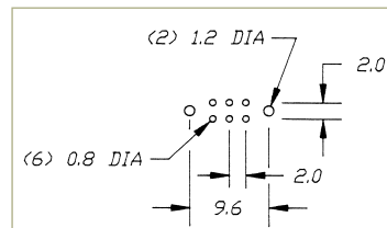
P.C. MOUNTING
