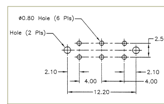
P.C. MOUNTING
