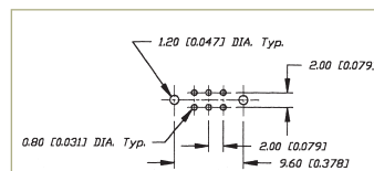
P.C. MOUNTING
