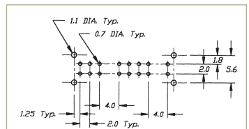
P.C. MOUNTING
