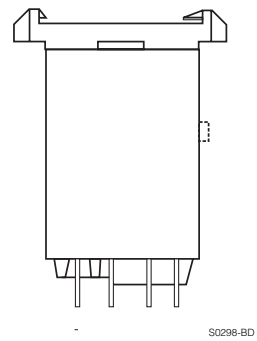
Cover with DIN-snap-on attachment (6.3 mm quick connect only) horizontal vertical
