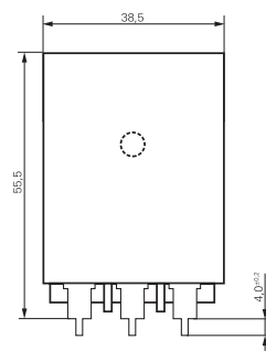
PCB version
