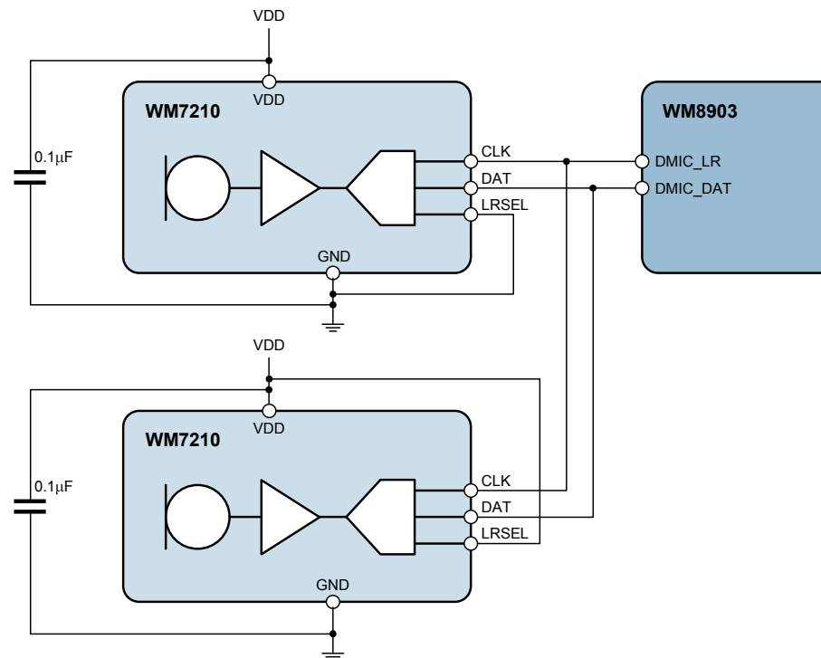
Figure 2 Stereo WM7210 Digital Microphone connection to WM8903
