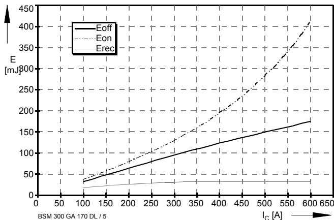
Bild / Fig. 5 Schaltverluste (typisch) / Switching losses (typical) E_{on} = f(I_C) , E_{off} = f(I_C) , E_{rec} = f(I_C) R_{gon} = R_{goff} = 5\Omega , V_{CE} = 900\text{V} , T_J = 125^\circ\text{C}
