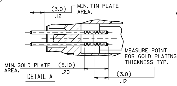
DIMENSIONS FOR SELECTIVE PLATING'S, SCALE 4:1
