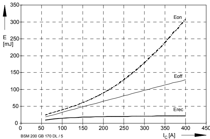
Bild / Fig. 5 Schaltverluste (typisch) / Switching losses (typical) E_{on} = f(I_C), E_{off} = f(I_C), E_{rec} = f(I_C) R_{\theta n} = R_{\theta ns} = 7.5\Omega, V_{CE} = 900V, T_i = 125^\circ C
