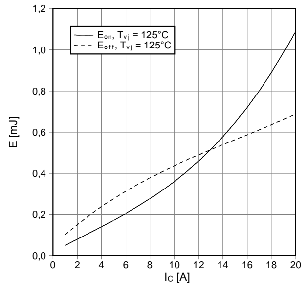
Schaltverluste IGBT-Wechselr. (typisch) switching losses IGBT-inverter (typical) E_{on} = f(I_c) , E_{off} = f(I_c) V_{GE} = \pm 15\text{ V} , R_{Gon} = 82\ \Omega , R_{Goff} = 82\ \Omega , V_{CE} = 300\text{ V}
