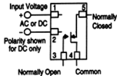
Single Pole - Double Throw
