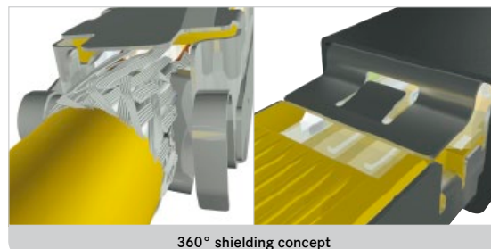
360° shielding concept
