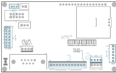
Figure 8: RS422 Connections
