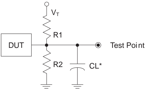
Figure 3-30. Output Test Load, LVTTTL and LVCMOS Standards
