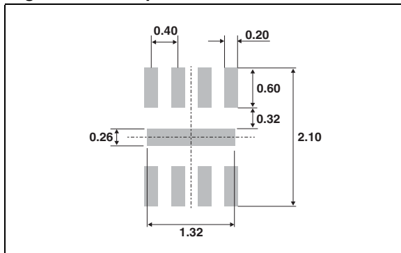
Figure 17. Footprint
