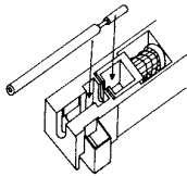
Drop bowden barrel into seat of switch
