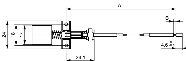
Type B (Screw-on mounting)
