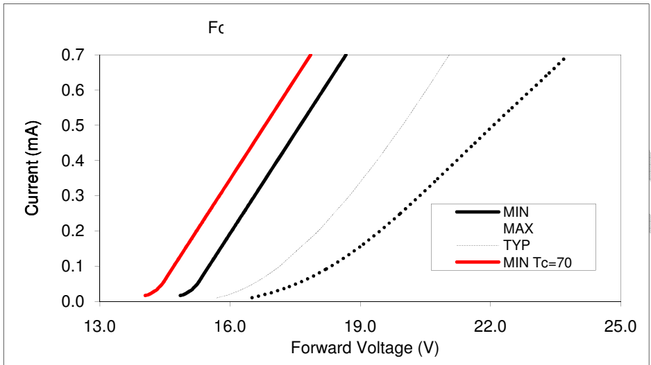
Figure 10: Typical Current vs. Voltage, BXR-XXX0540-A, BXR-56C0700-A
