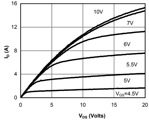
Figure 2: On-Region Characteristics @ 125°C
