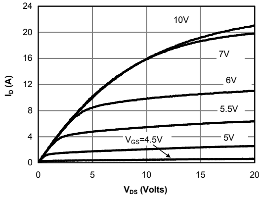
Figure 1: On-Region Characteristics @ 25°C
