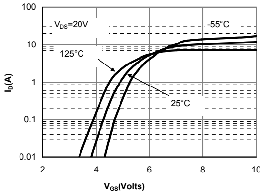
Figure 3: Transfer Characteristics
