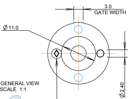
DIAMOND DOWEL SEE DETAIL C
