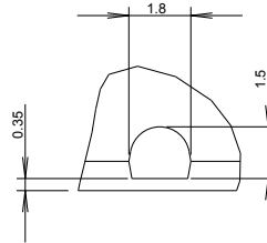
DETAIL B SCALE 8:1
